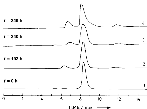
Figure 7. HPLC traces for the cleavage of 2',3'-cAMP at pH 8.0 and 30 °C. 1: 2',3'-cAMP; 2: cleavage of 2',3'-cAMP by template 2 ; 3: cleavage of 2',3'-cAMP by template 1 ; 4: recycled template 1 . Retention times: 3'-AMP 6.91 min; 2',3'-cAMP 8.33 min; 2'-AMP 11.95 min.
