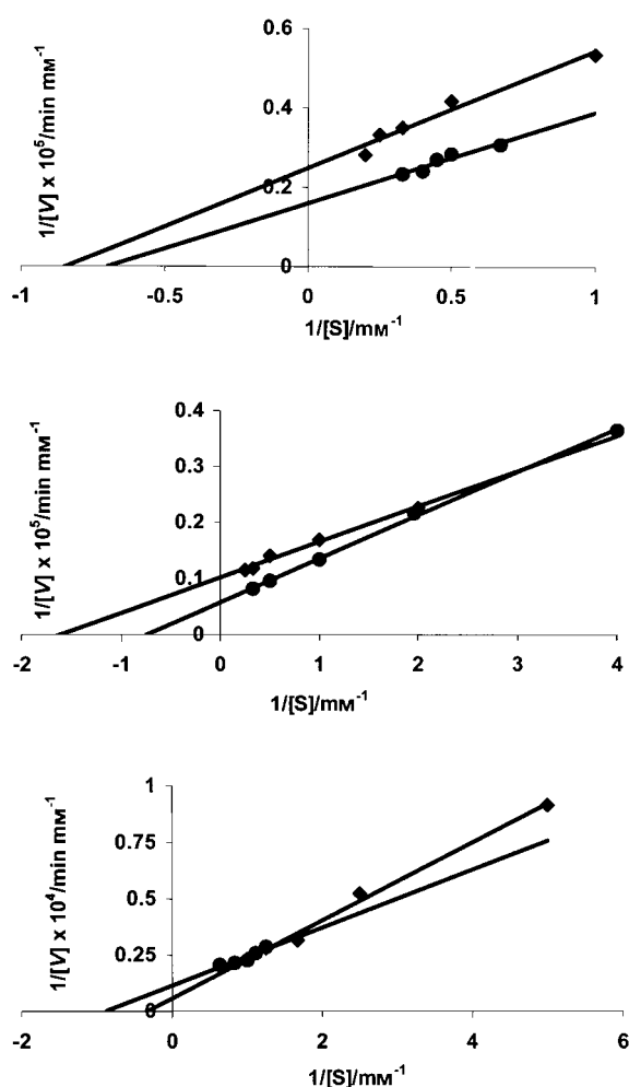
Figure 6. Lineweaver–Burk plots for hydrolysis of p NPP (top), b NPP (middle), and h NPP (bottom) by templates 1 (◆) and 2 (●).
