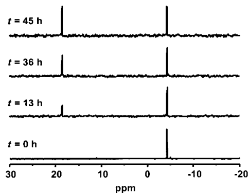
Figure 8. ^{31}\text{P} NMR spectra for the hydrolysis of hNPP by template 2 . Chemical shifts for hNPP and for the cyclic phosphate product are -4.32 ppm and 18.58 ppm, respectively. [21d] The chemical shifts are with respect to 85\% \text{H}_3\text{PO}_4 as external reference.
