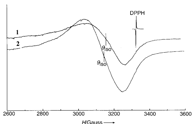
Figure 1. Solid-state EPR spectra for templates 1 and 2 at room temperature.
