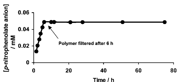
Figure 9. Reaction arrest experiment for bNPP hydrolysis by template 2 .
