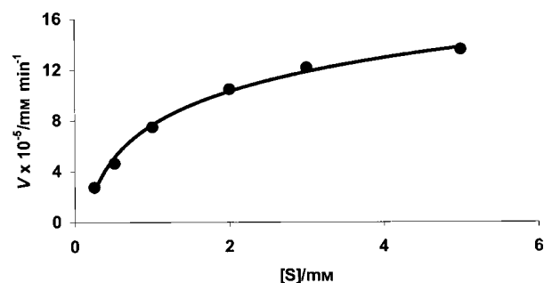
Figure 5. Michaelis–Menten saturation kinetics for bNPP hydrolysis catalyzed by template 2 .
