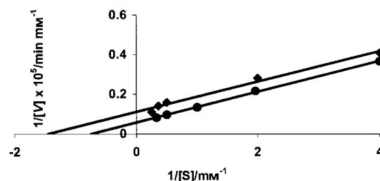
Figure 10. Lineweaver–Burk plots for bNPP hydrolysis by template 2 : (●) in absence of inhibitor; (◆) in the presence of inhibitor.
