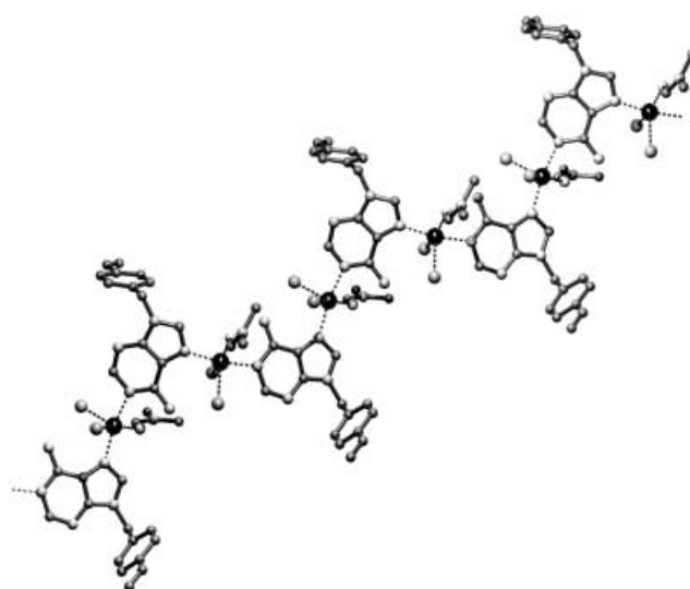
Figure 3. POVray diagram showing the polymeric structure of the 9VBA-Cu complex. Hydrogen atoms are omitted for clarity.
