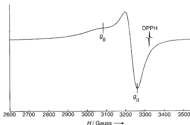
Figure 4. Solid-state EPR spectrum of the 9VBA-Cu complex.
