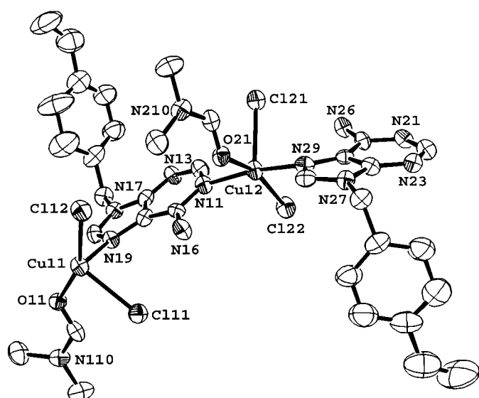
Figure 2. POVray-rendered ORTEP diagram showing the asymmetric unit of 9VBA-Cu complex. Hydrogen atoms are excluded for clarity.
